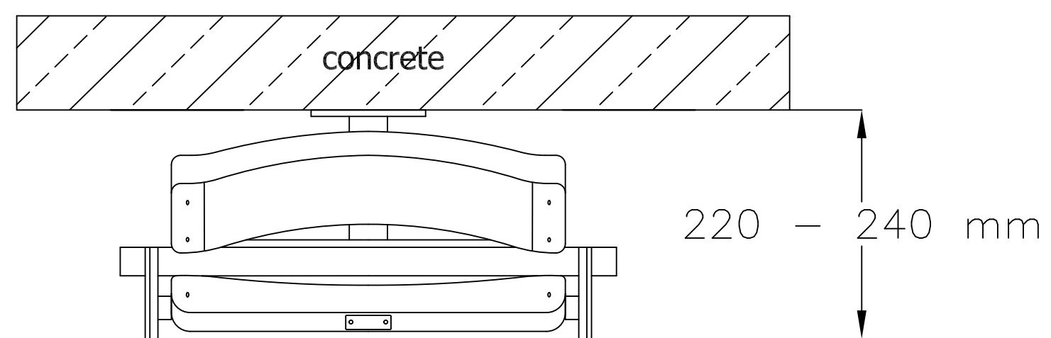
TOP VIEW
