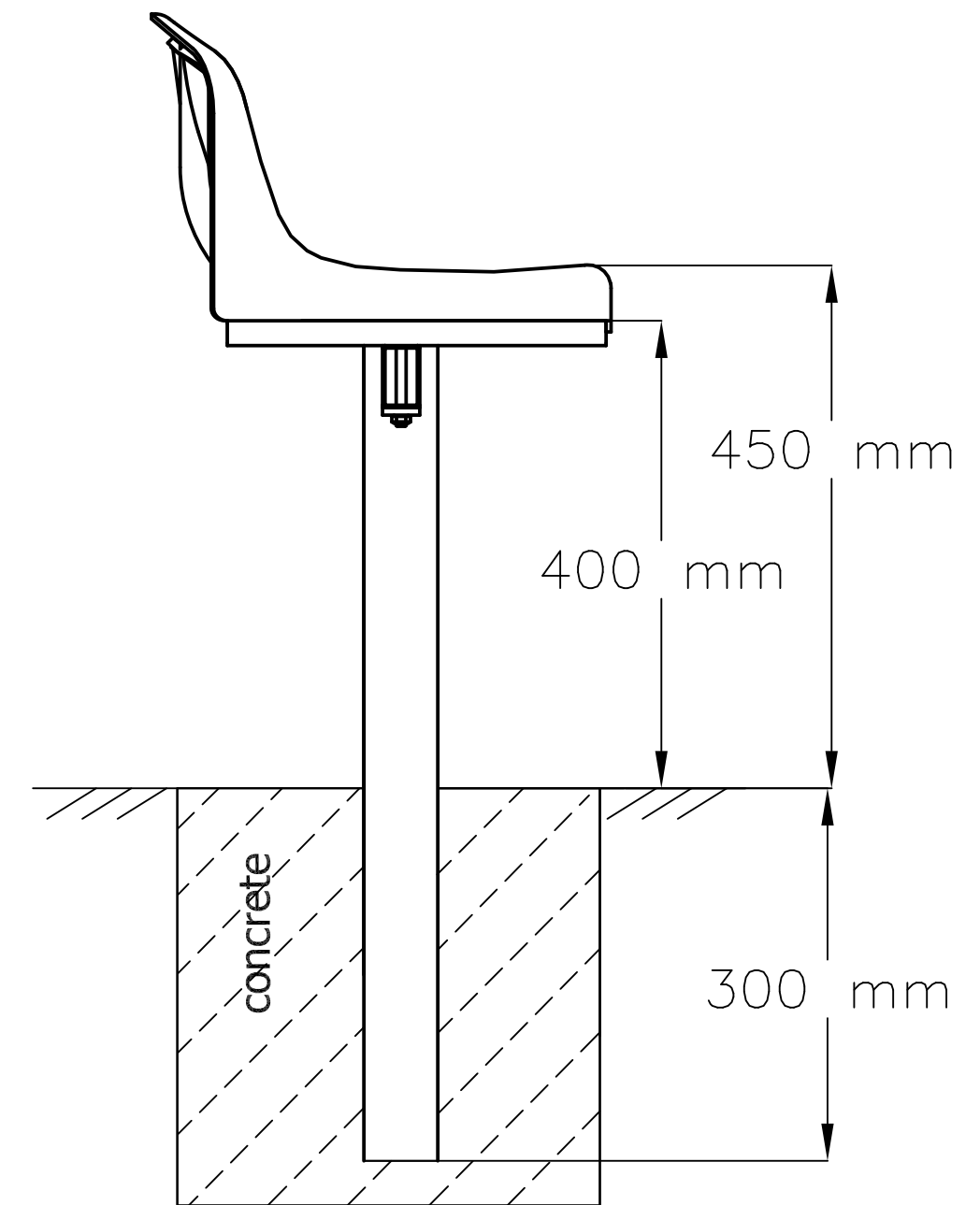
SIDE VIEW
