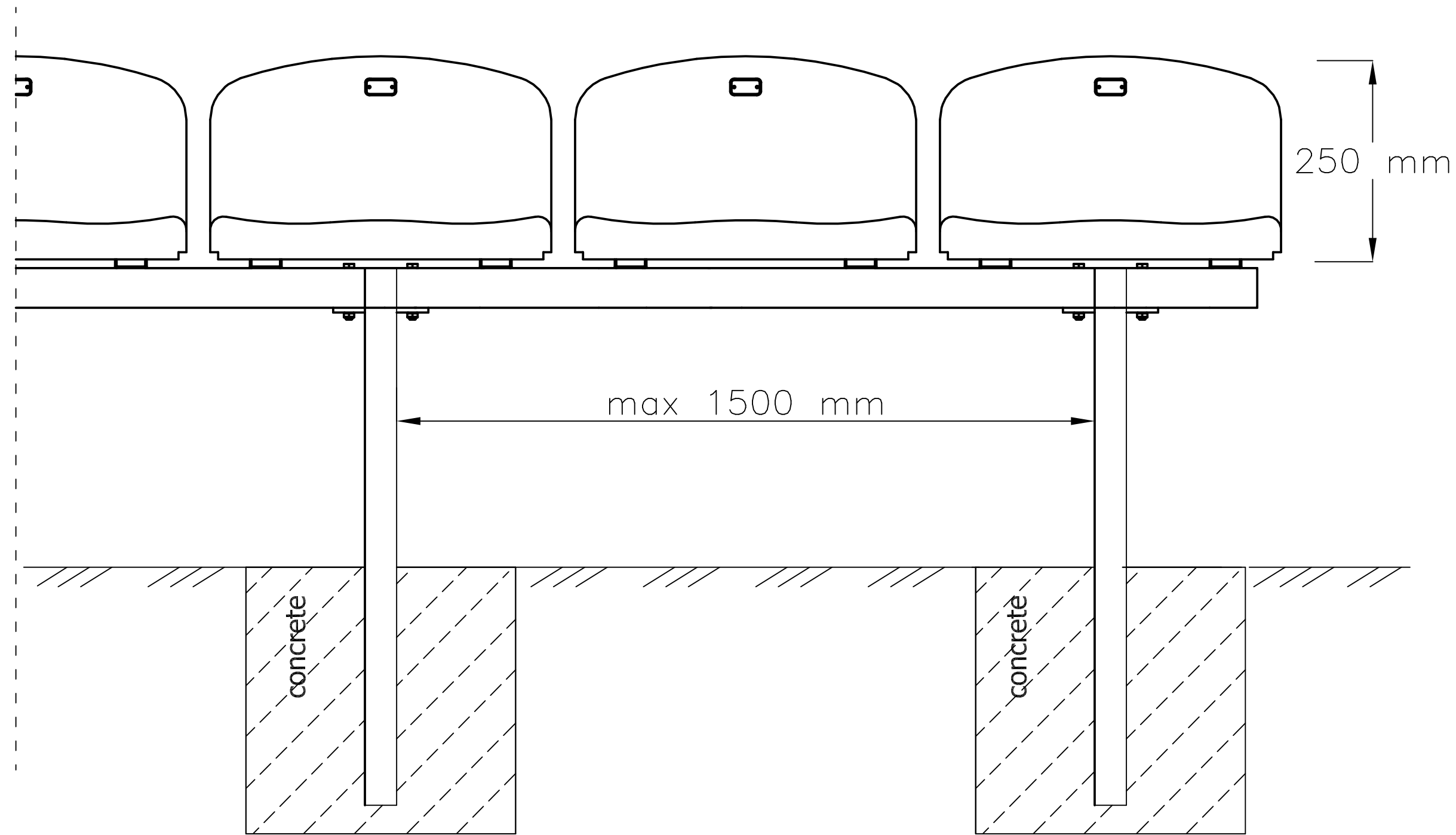
FRONT VIEW
