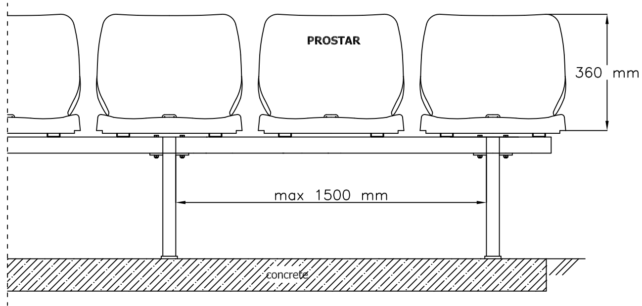
FRONT VIEW
